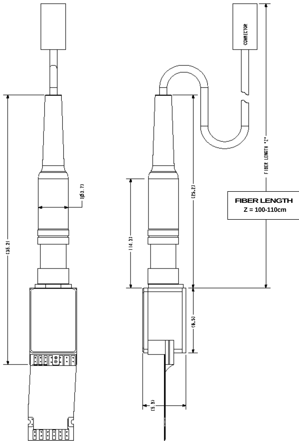
Fiber Pigtailed Version detail (162xFxx):
